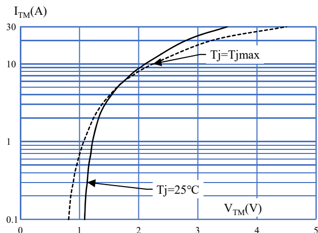
FIG.4: On-state haracteristics(maximum values)
