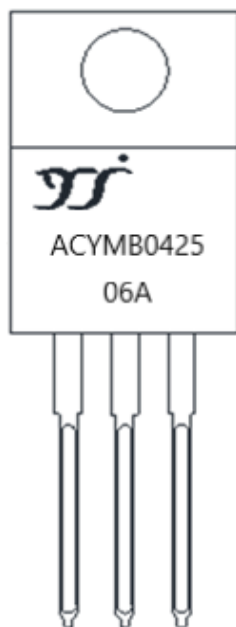
(TO-220AB-1 Package)
